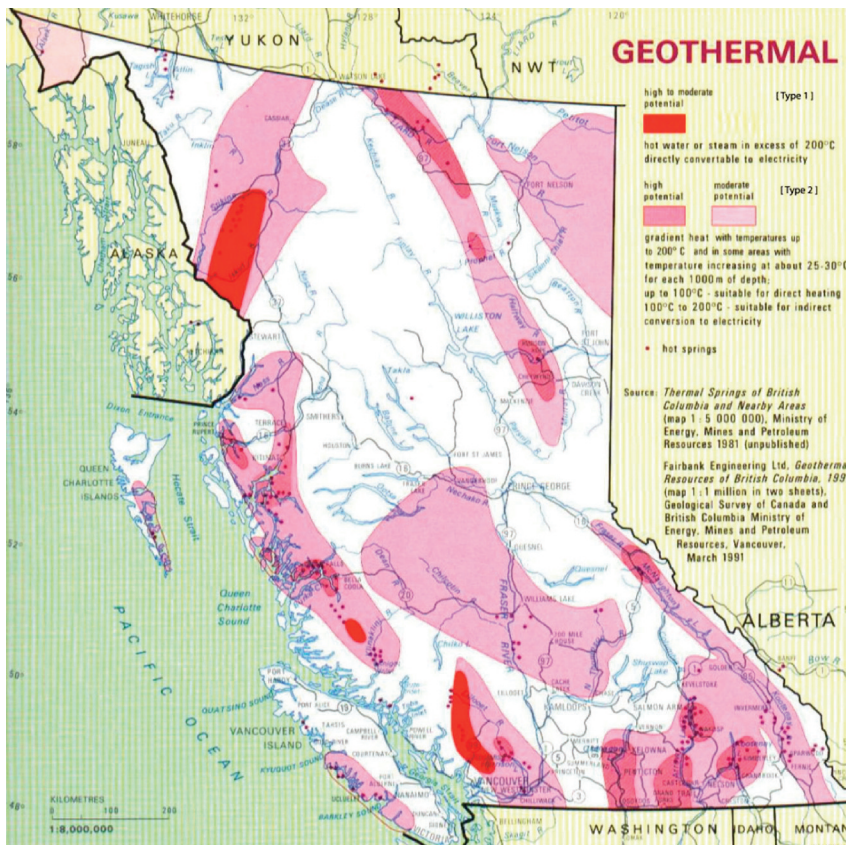
Figure 1: Map of geothermal resources in British Columbia. Source: Fairbank Engineering Ltd. 1991.
