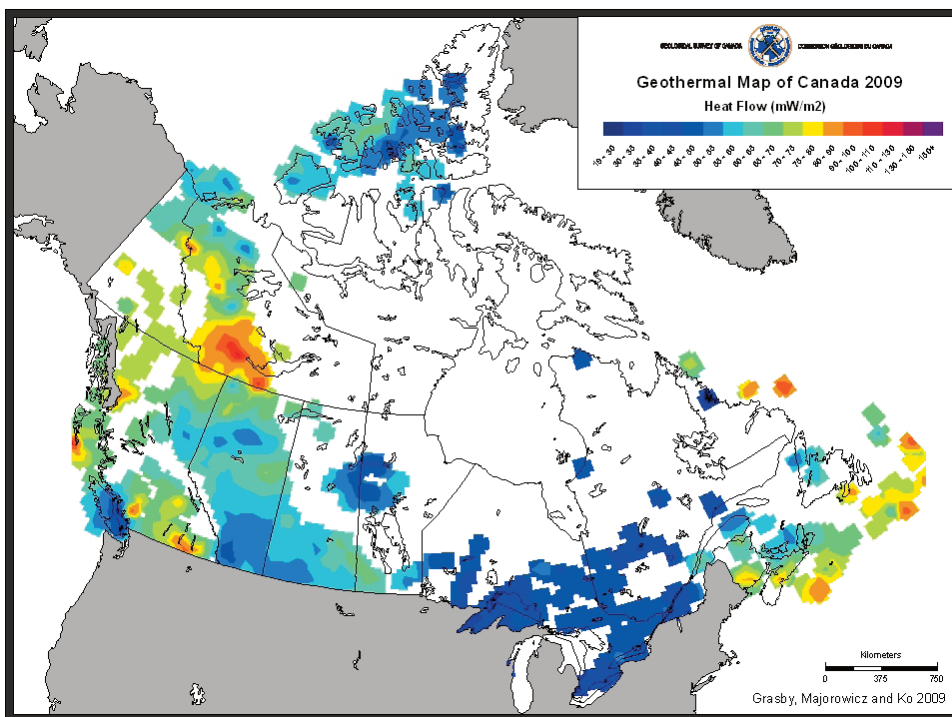
Figure 2: Geothermal map of Canada Source: Grasby et al. 2009
